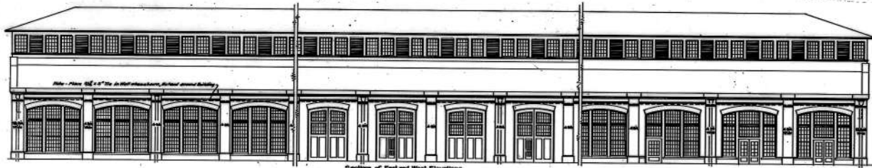
Section of East and West Elevations.
