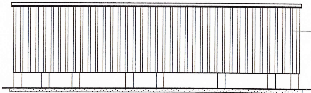
1 x 4 Board and Batten Siding, 11 1/2" on center, front and rear, 12" o.c. on sides, painted white.
